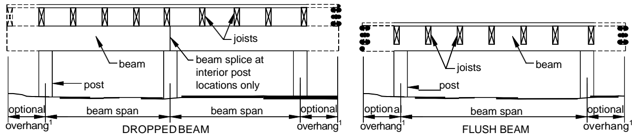
Figure 3 BEAM TYPES
