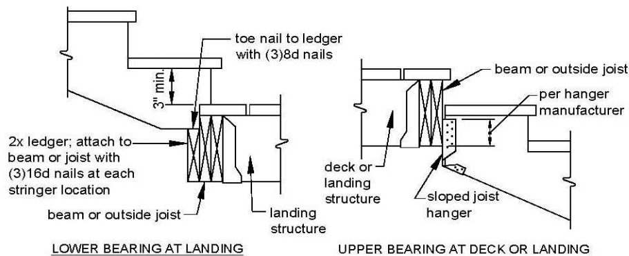
Figure 28 STRINGER BEARING
