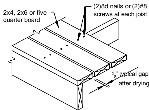
Figure 22 TYPICAL DECKING
