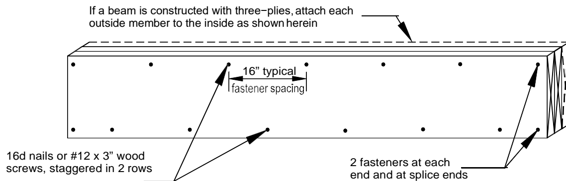
Figure 4 BEAM ASSEMBLY
