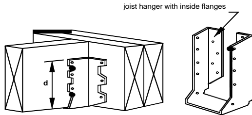
Figure 9 JOIST HANGERS
